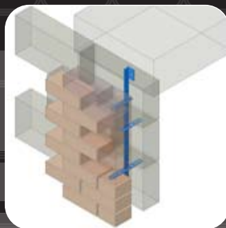
Type JPA/F Fixed to the edge of a slab
