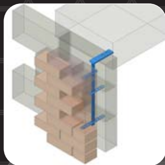
Type JPA/L Fixed to a soffit frame
