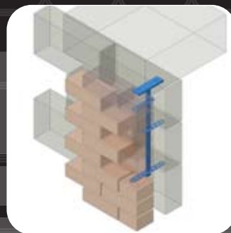
Type JPA/T Fixed to a soffit frame
